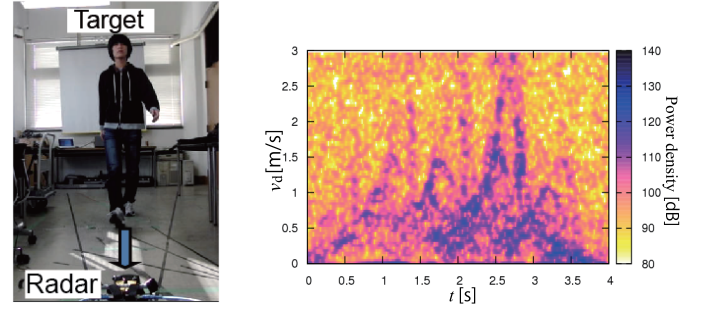
(a) Experimental site (b) Summation of the spectrograms for range bins Fig. 2. Experimental setup and spectrogram at z_c = 0.36 m of a pedestrian.
