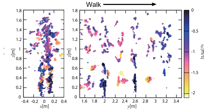
Fig. 5. Frontal (left) and side views (right) of the estimated image of a pedestrian walking away from the radar along the y -axis.
