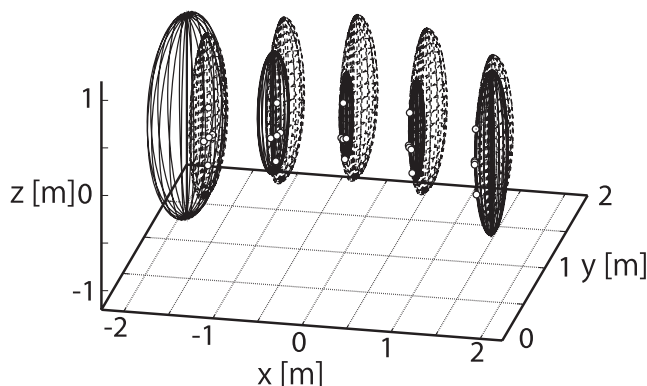
Fig. 7 Actual target shapes (dashed lines) and estimated ellipsoidal model shapes (solid lines) for an asymmetrical target.
